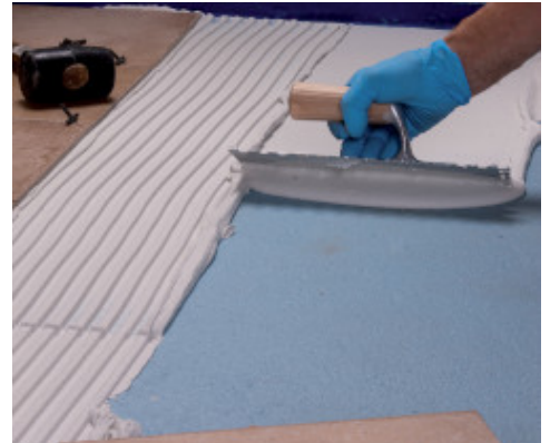
Bonding tiles on Mapelastc AquaDefense
